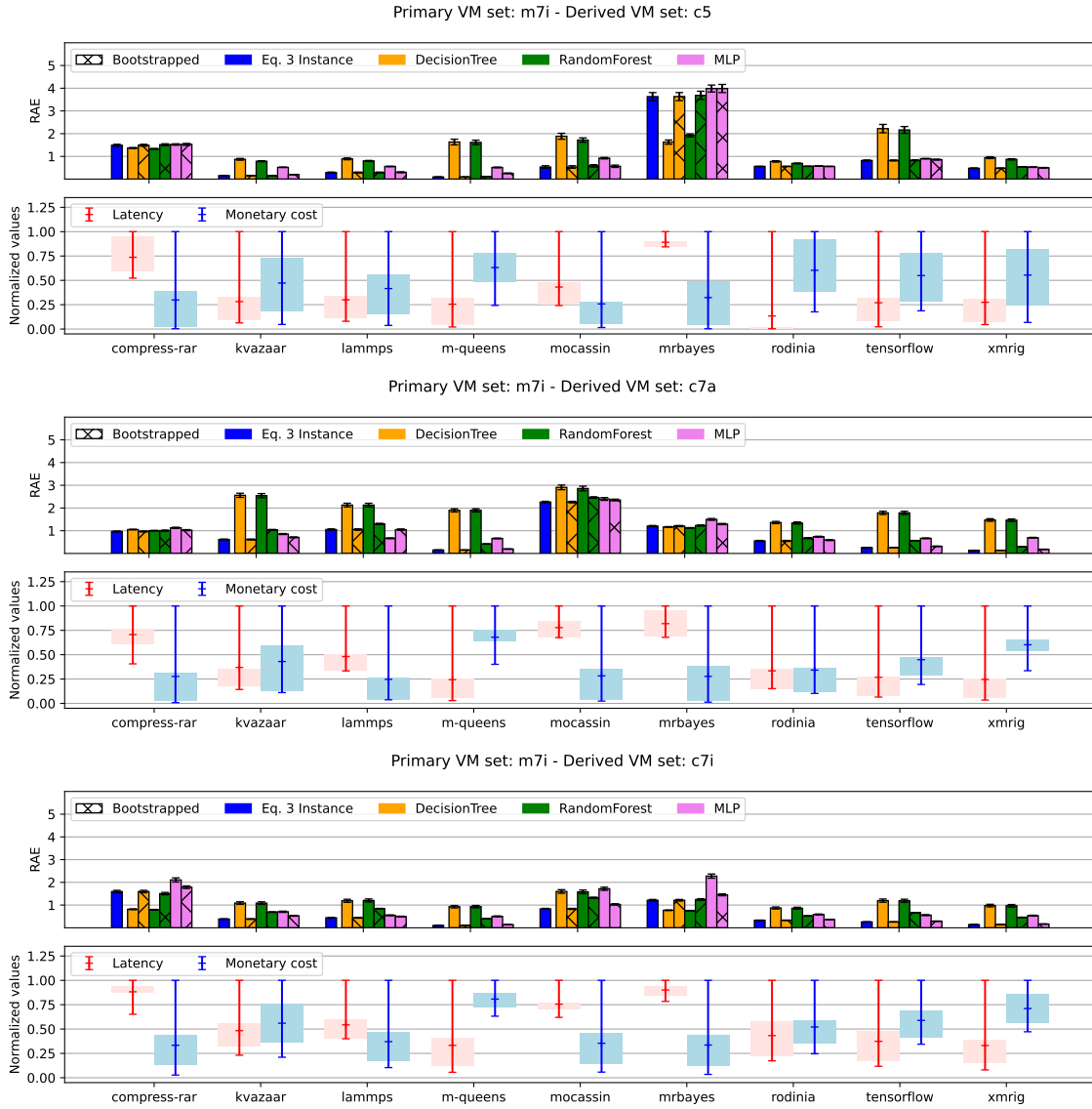
Fig. 8. Results for C5, C7a and C7i families for all benchmark applications, using M7i family as a primary VM set, three samples ( k = 3 ) for the primary VM set and one sample for each.
